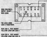
FIGURE I. TRANSFORMER (PART OF POWER—TRANSFORMER MODULE A2, LOCATED IN BACK BOX).
