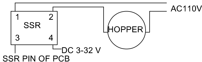
Hopper Connection Diagram
