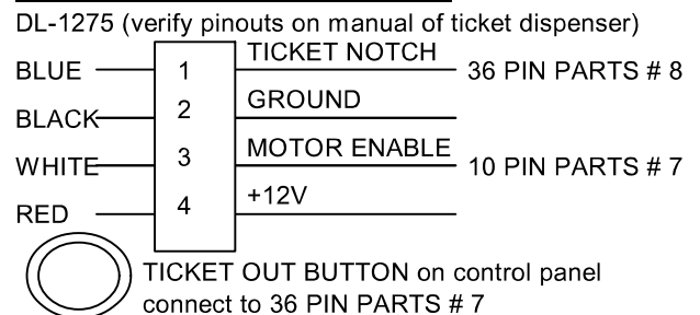
Ticket Dispenser Connection Diagram
