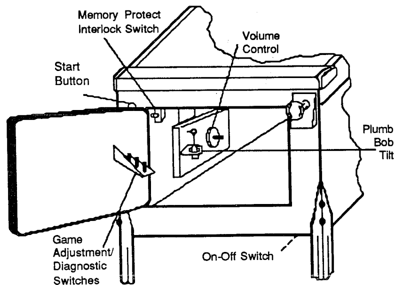
Figure 2. Control Locations
