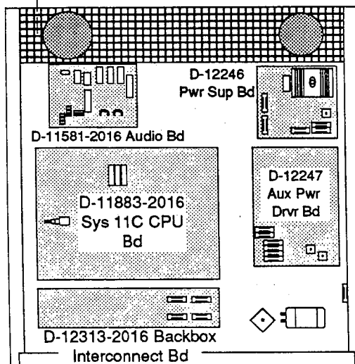
Backbox
