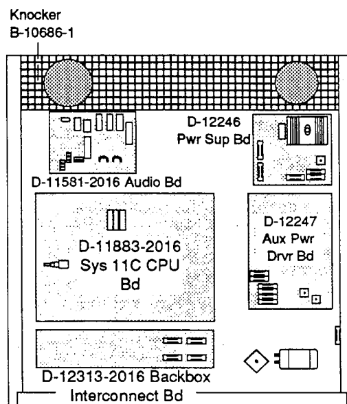
Backbox
